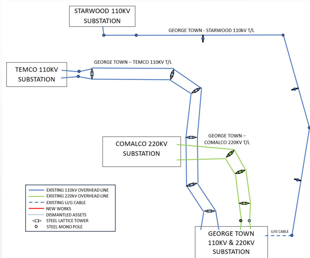
Figure 5: Overview of existing network
